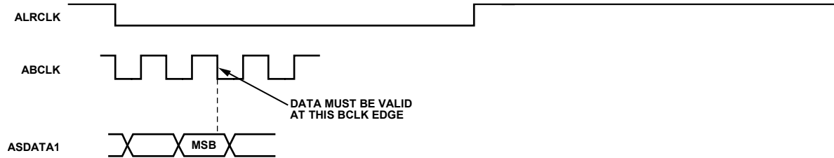
Figure 16. 1 st S Pipeline Mode in ADC Serial Data Transmission (Applicable in Stereo and TDM Useful for High Frequency TDM Transmission)
